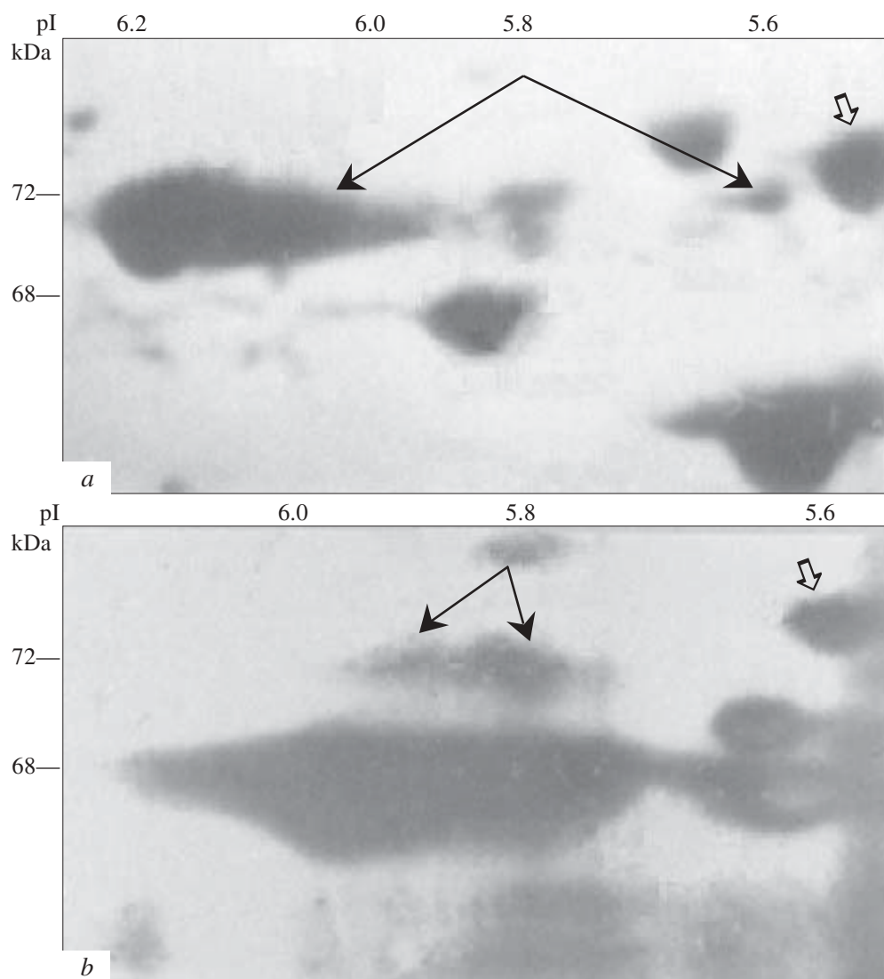
Fig. 3. Fragments of gels corresponding to location of HSP70 stress proteins after 2D-electrophoresis of cytoplasmic myocardial proteins. a ) myocardium of a rat exposed to heat shock; b ) biopsy specimen of the atrium from a coronary patient with pronounced dyskinesia of the heart. Arrow shows inducible stress proteins; double arrow shows constitutive stress proteins.
